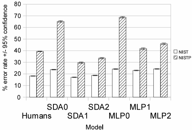
NIST 62 character classes (humans, MLPs, SDAs)
