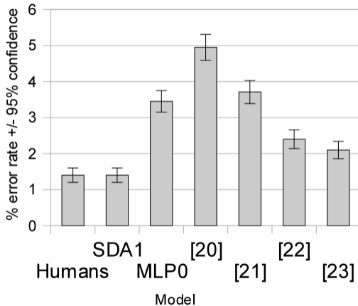
NIST digits, machines vs humans
