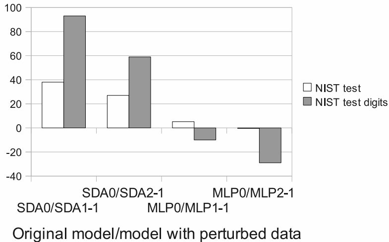
Relative change in error rate Due to the use of perturbed data
