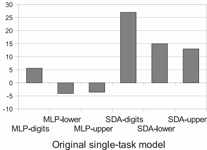
Relative improvement due to use of multi-task setting
